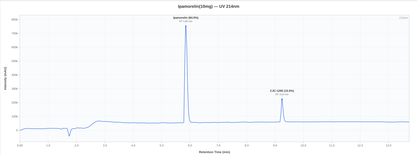
Representative chromatogram, Conformity V2 (closest to batch mean purity)
